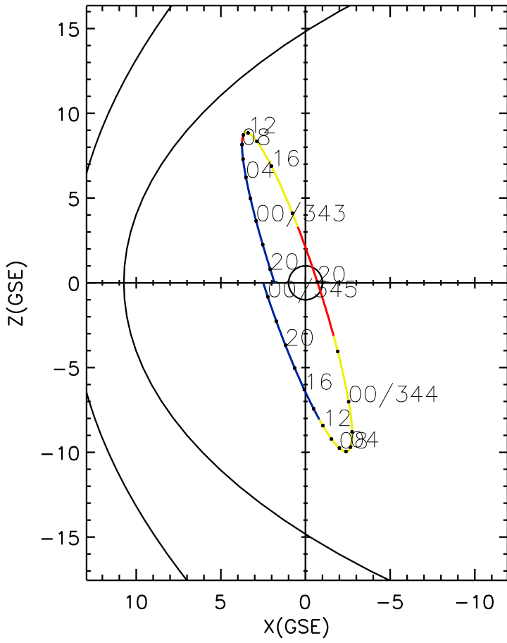
CLUSTER 2 orbit 2017 342 (12/08) 18:51 UT to 2017 345 (12/11) 01:06 UT
