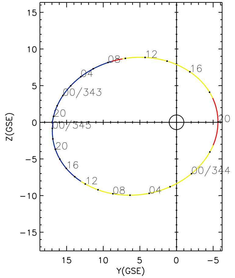
CLUSTER 2 orbit 2017 342 (12/08) 18:51 UT to 2017 345 (12/11) 01:06 UT
