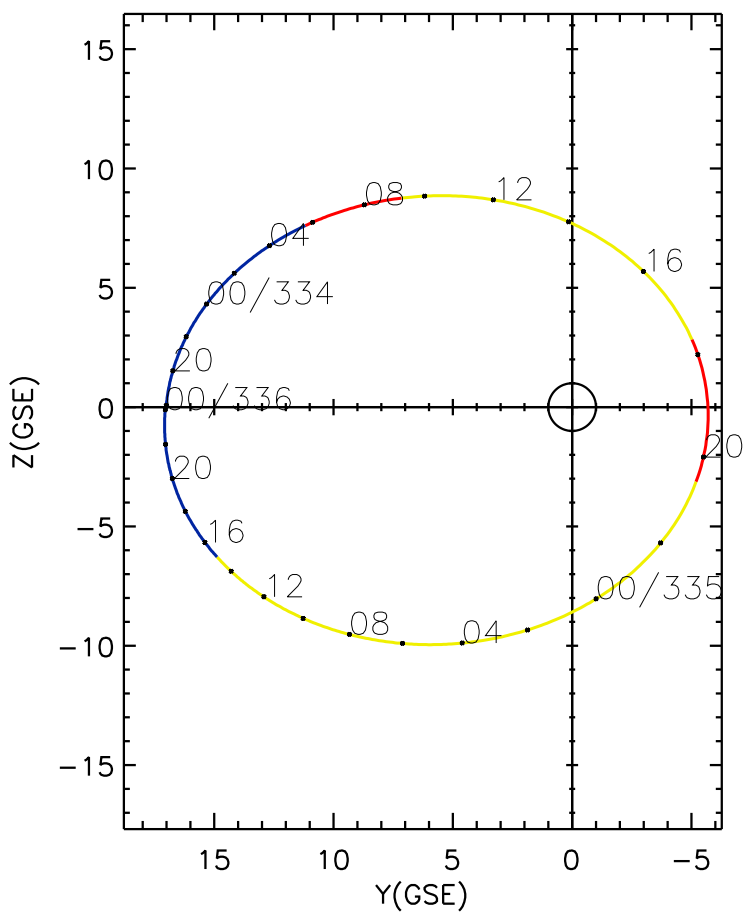
CLUSTER 2 orbit 2017 333 (11/29) 17:51 UT to 2017 336 (12/02) 00:06 UT
