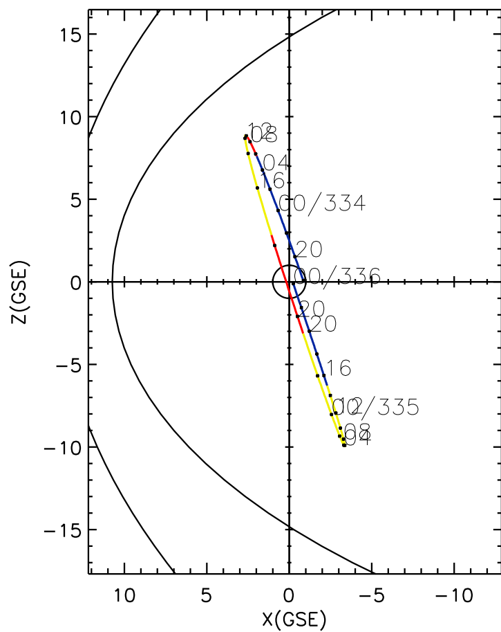
CLUSTER 2 orbit 2017 333 (11/29) 17:51 UT to 2017 336 (12/02) 00:06 UT
