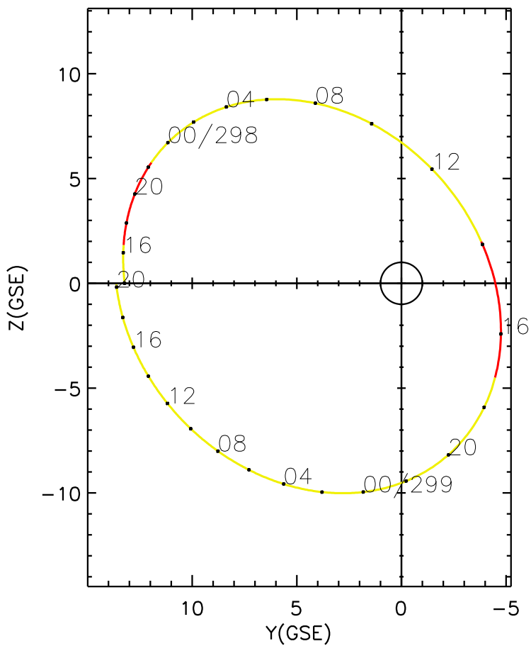
CLUSTER 2 orbit 2017 297 (10/24) 13:56 UT to 2017 299 (10/26) 20:11 UT
