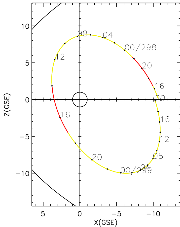
CLUSTER 2 orbit 2017 297 (10/24) 13:56 UT to 2017 299 (10/26) 20:11 UT
