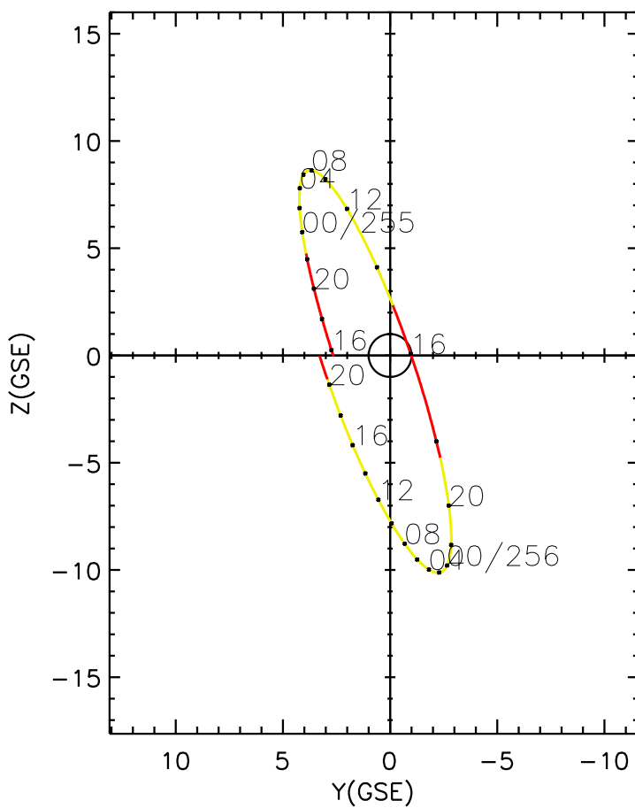
CLUSTER 2 orbit 2017 254 (09/11) 15:36 UT to 2017 256 (09/13) 21:51 UT
