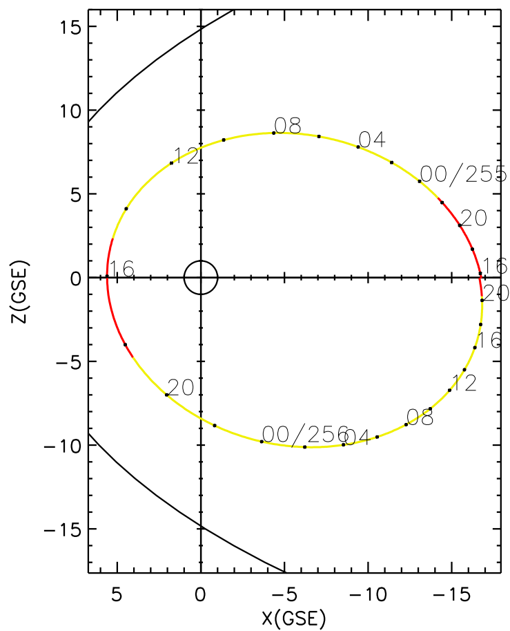
CLUSTER 2 orbit 2017 254 (09/11) 15:36 UT to 2017 256 (09/13) 21:51 UT
