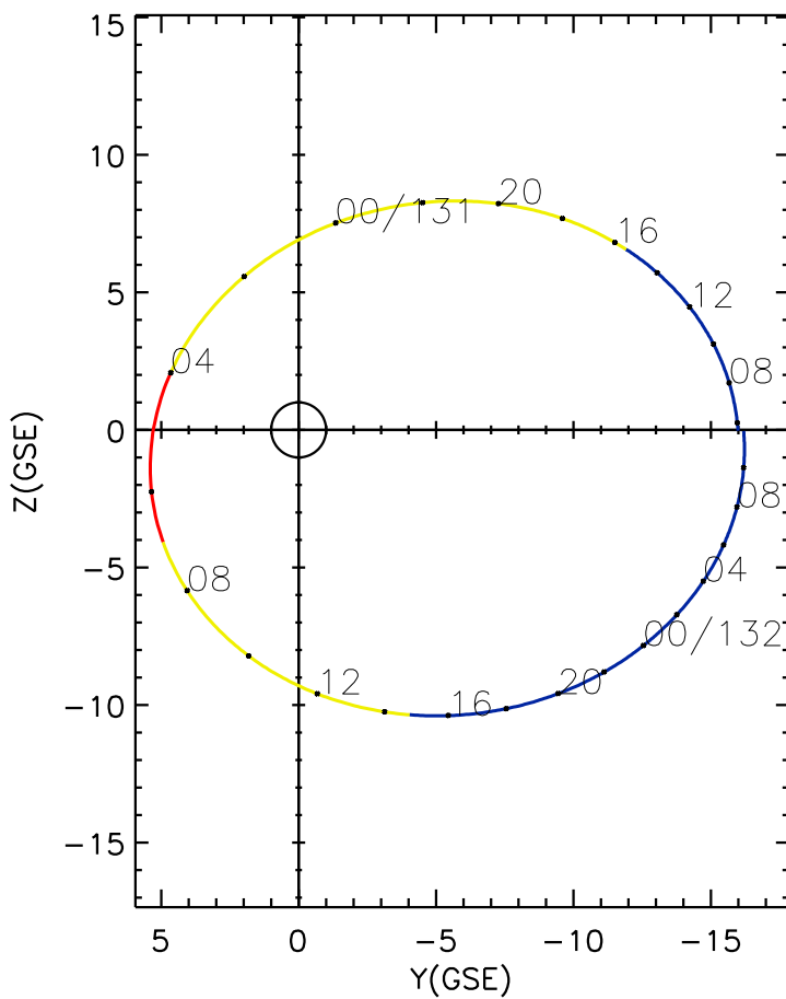
CLUSTER 2 orbit 2017 130 (05/10) 05:36 UT to 2017 132 (05/12) 11:51 UT
