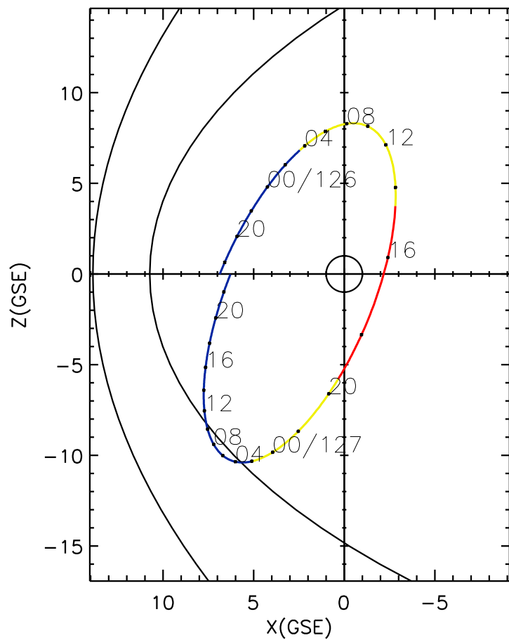
CLUSTER 2 orbit 2017 125 (05/05) 17:06 UT to 2017 127 (05/07) 23:21 UT
