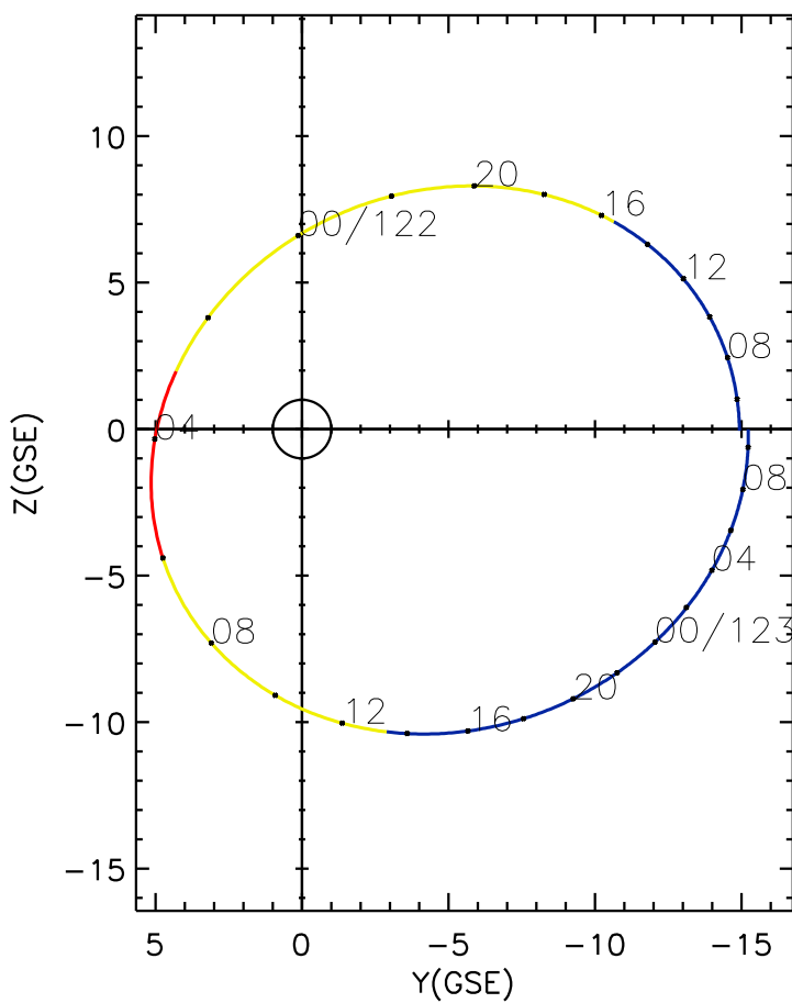
CLUSTER 2 orbit 2017 121 (05/01) 04:31 UT to 2017 123 (05/03) 10:51 UT
