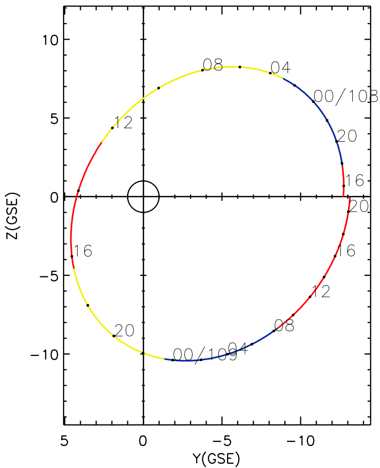
CLUSTER 2 orbit 2017 107 (04/17) 15:01 UT to 2017 109 (04/19) 21:16 UT
