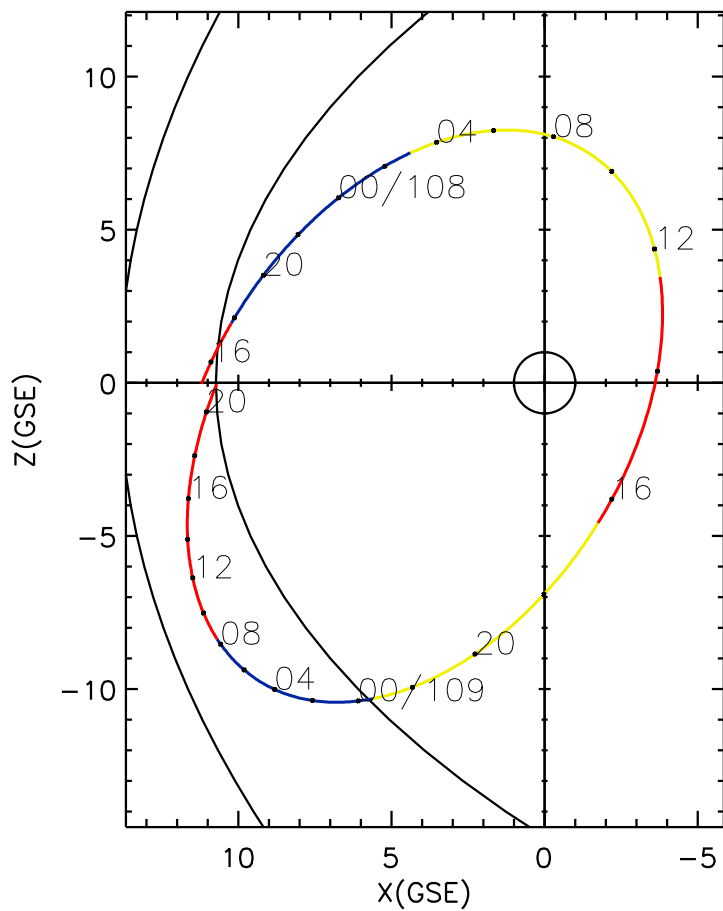
CLUSTER 2 orbit 2017 107 (04/17) 15:01 UT to 2017 109 (04/19) 21:16 UT
