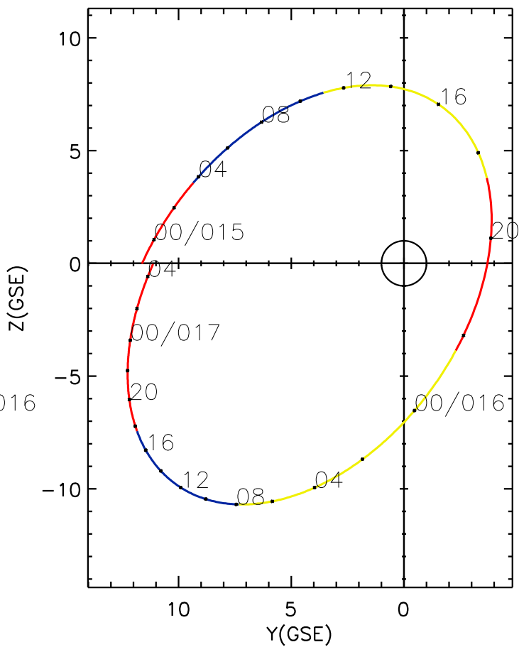
CLUSTER 2 orbit 2017 014 (01/14) 22:31 UT to 2017 017 (01/17) 04:46 UT
