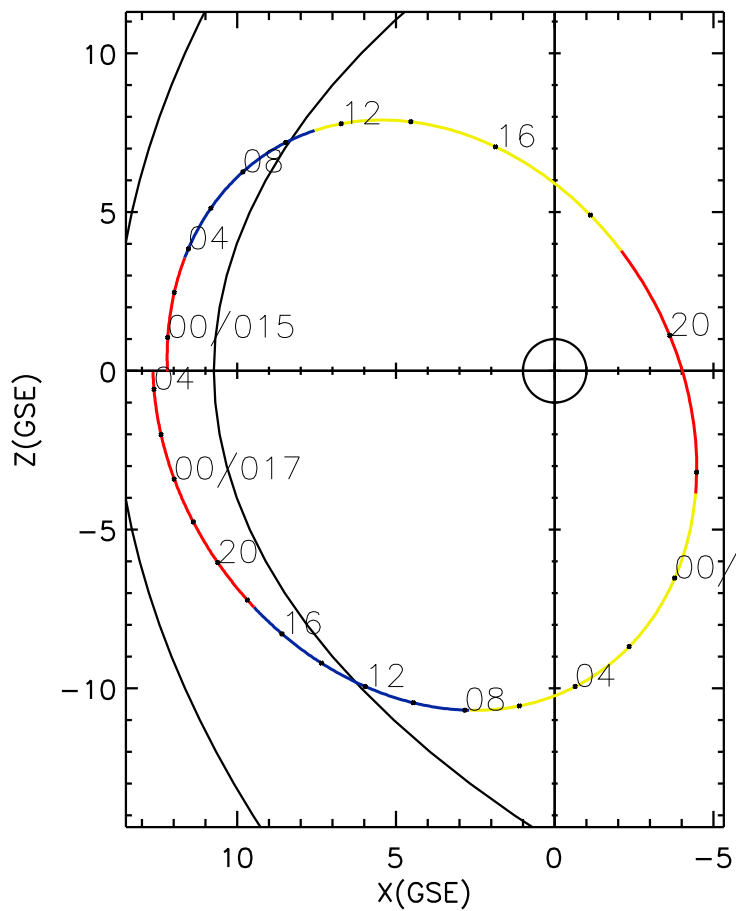
CLUSTER 2 orbit 2017 014 (01/14) 22:31 UT to 2017 017 (01/17) 04:46 UT
