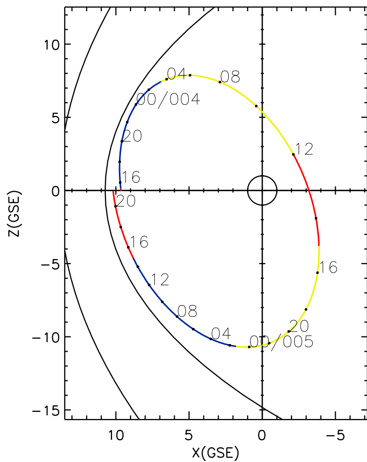
CLUSTER 2 orbit 2017 003 (01/03) 15:11 UT to 2017 005 (01/05) 21:26 UT
