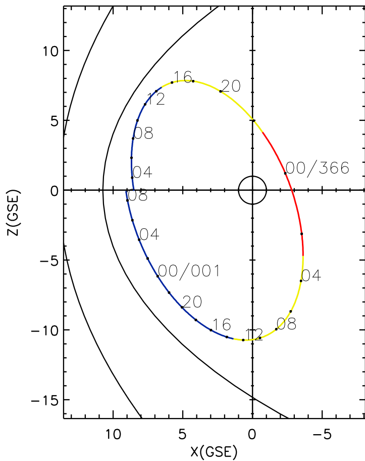
CLUSTER 2 orbit 2016 365 (12/30) 02:41 UT to 2017 001 (01/01) 08:56 UT
