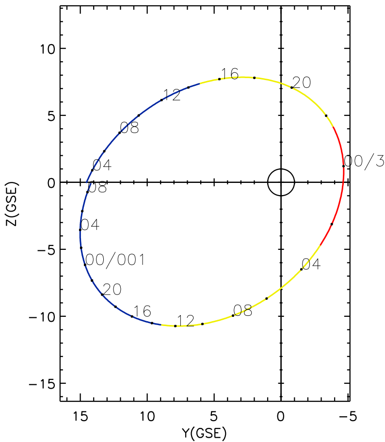
CLUSTER 2 orbit 2016 365 (12/30) 02:41 UT to 2017 001 (01/01) 08:56 UT
