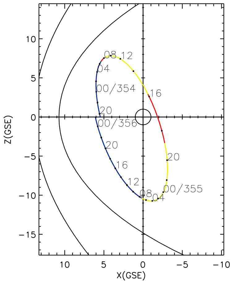
CLUSTER 2 orbit 2016 353 (12/18) 19:21 UT to 2016 356 (12/21) 01:41 UT
