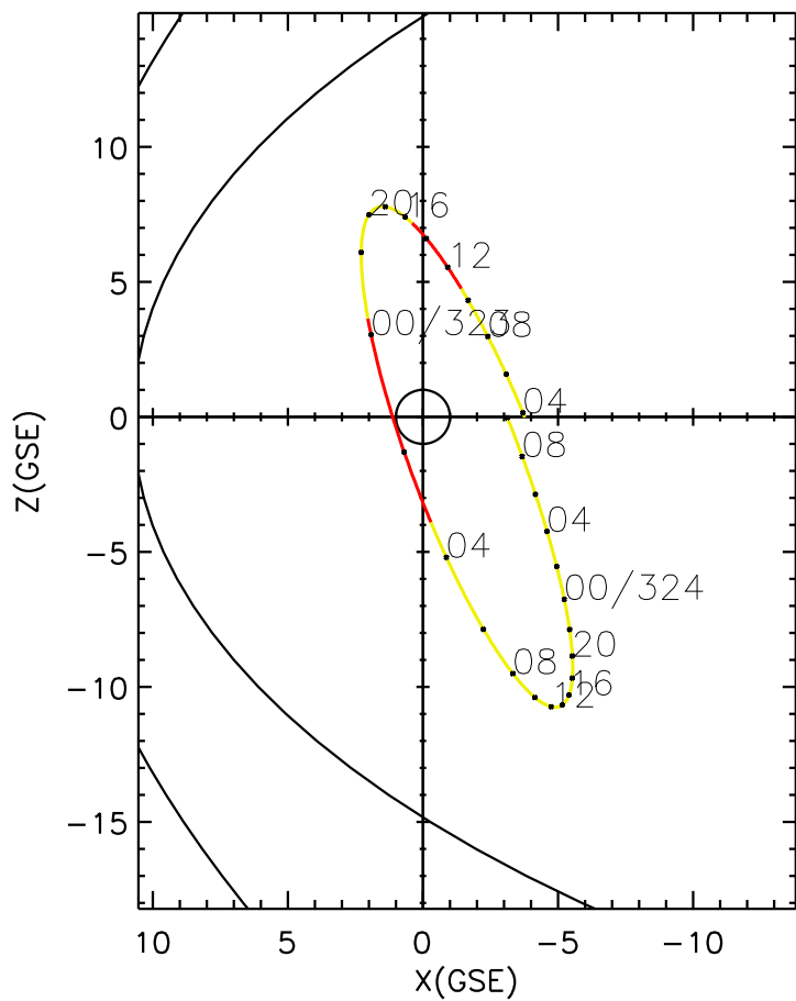
CLUSTER 2 orbit 2016 322 (11/17) 03:46 UT to 2016 324 (11/19) 10:01 UT
