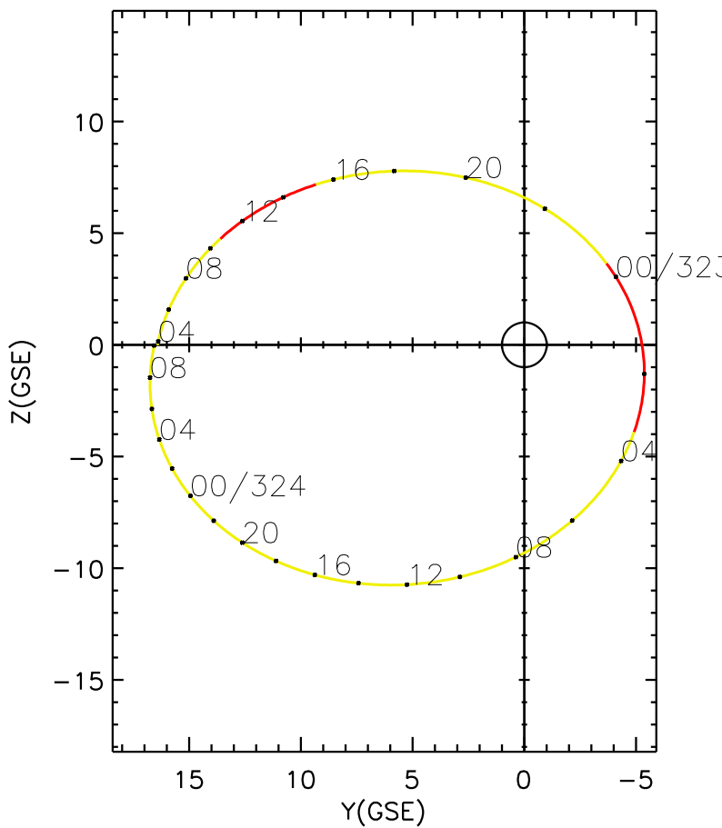
CLUSTER 2 orbit 2016 322 (11/17) 03:46 UT to 2016 324 (11/19) 10:01 UT
