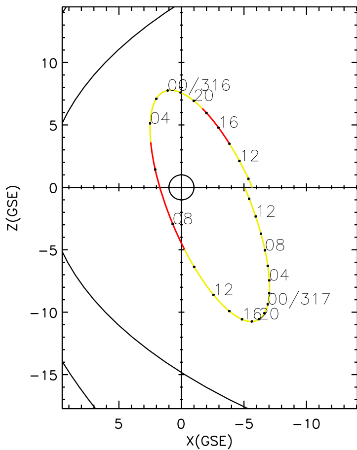
CLUSTER 2 orbit 2016 315 (11/10) 09:01 UT to 2016 317 (11/12) 15:11 UT
