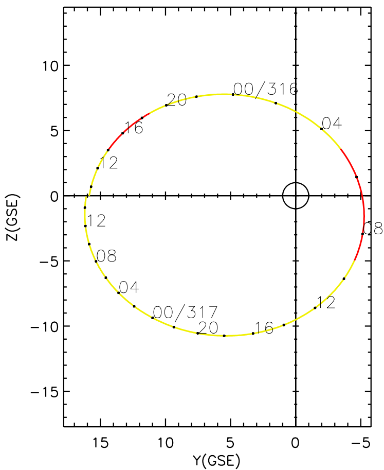
CLUSTER 2 orbit 2016 315 (11/10) 09:01 UT to 2016 317 (11/12) 15:11 UT
