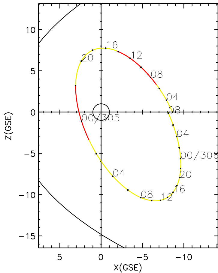
CLUSTER 2 orbit 2016 304 (10/30) 01:56 UT to 2016 306 (11/01) 08:11 UT
