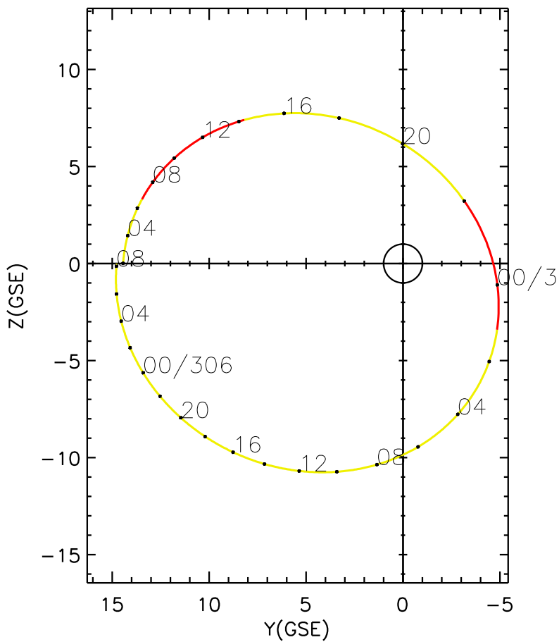
CLUSTER 2 orbit 2016 304 (10/30) 01:56 UT to 2016 306 (11/01) 08:11 UT
