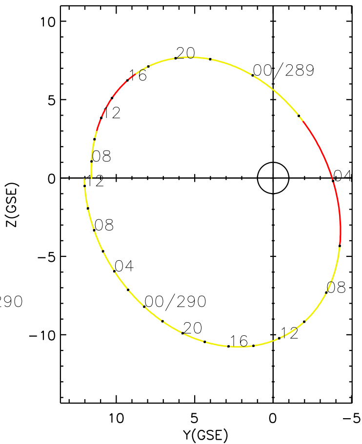
CLUSTER 2 orbit 2016 288 (10/14) 06:26 UT to 2016 290 (10/16) 12:41 UT
