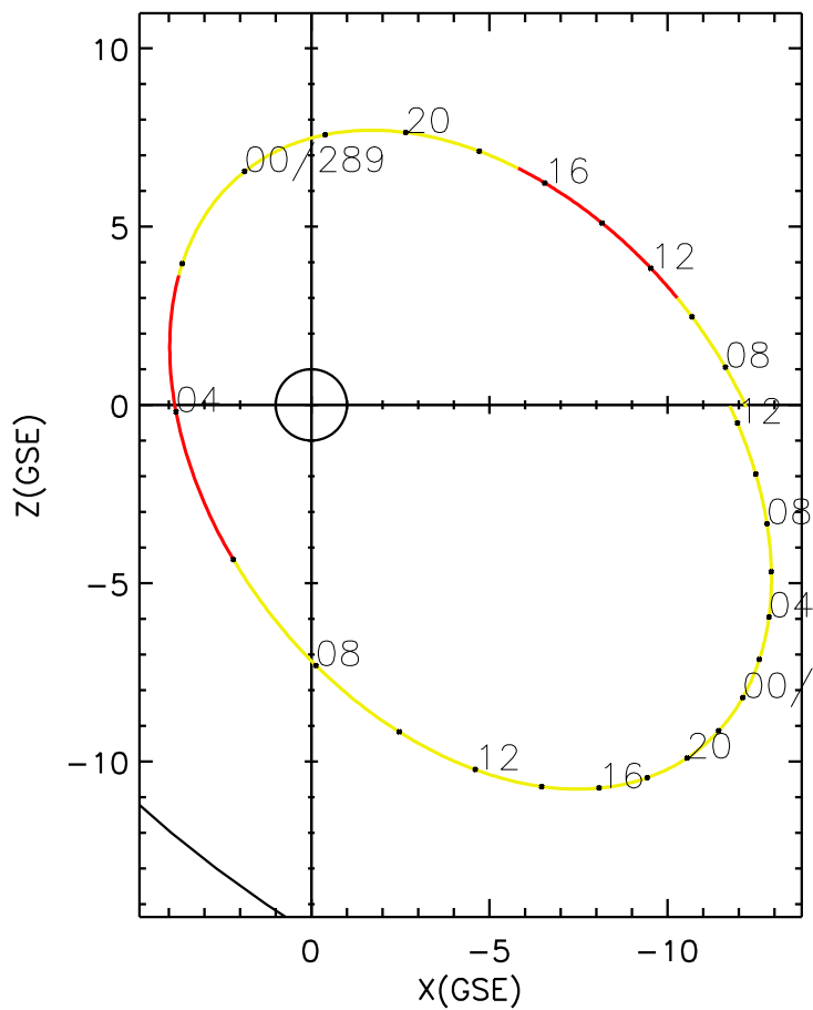
CLUSTER 2 orbit 2016 288 (10/14) 06:26 UT to 2016 290 (10/16) 12:41 UT
