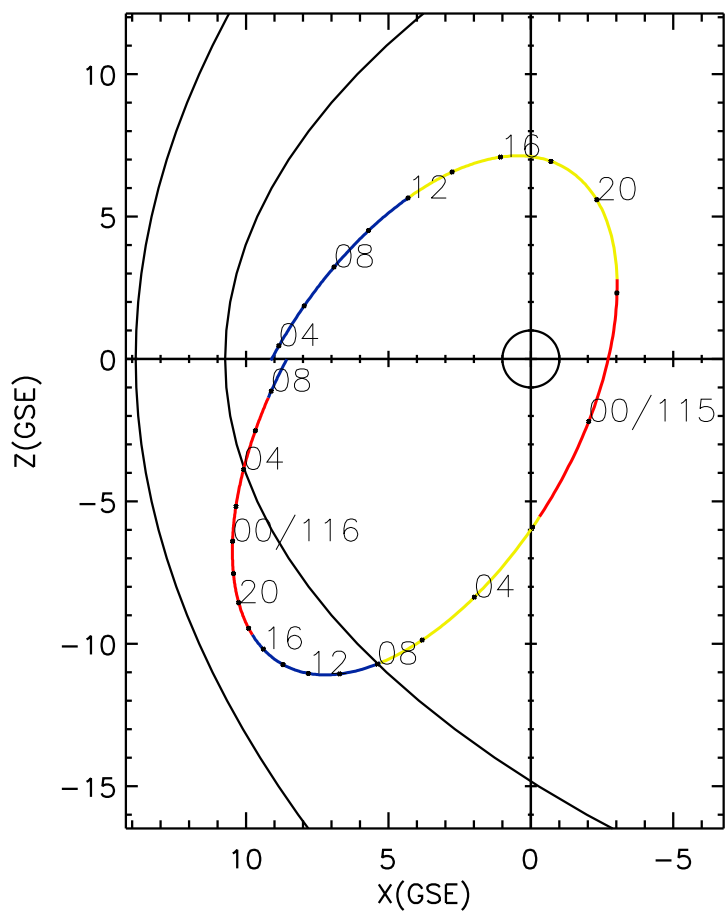
CLUSTER 2 orbit 2016 114 (04/23) 03:16 UT to 2016 116 (04/25) 09:36 UT
