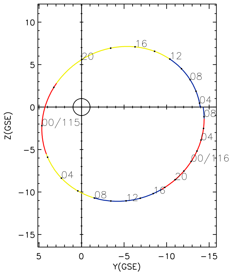
CLUSTER 2 orbit 2016 114 (04/23) 03:16 UT to 2016 116 (04/25) 09:36 UT
