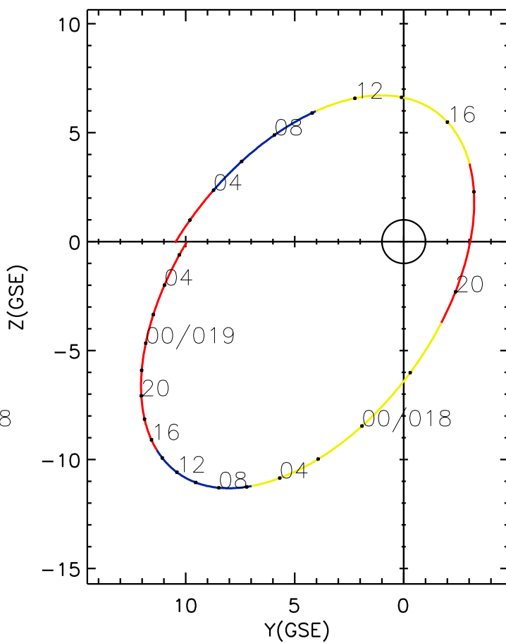
CLUSTER 2 orbit 2016 017 (01/17) 00:31 UT to 2016 019 (01/19) 06:51 UT
