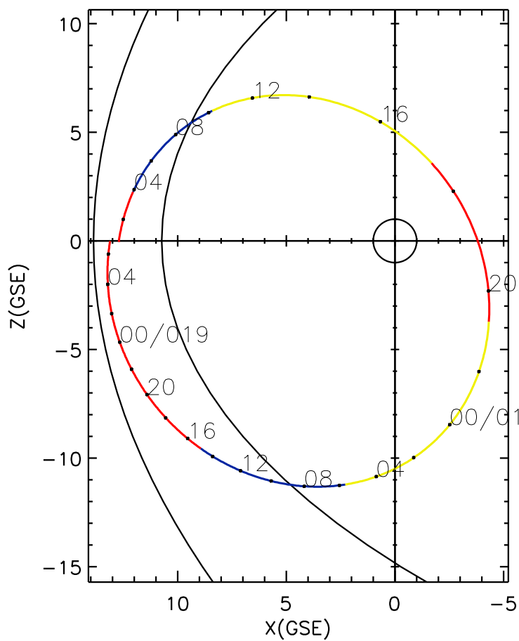
CLUSTER 2 orbit 2016 017 (01/17) 00:31 UT to 2016 019 (01/19) 06:51 UT
