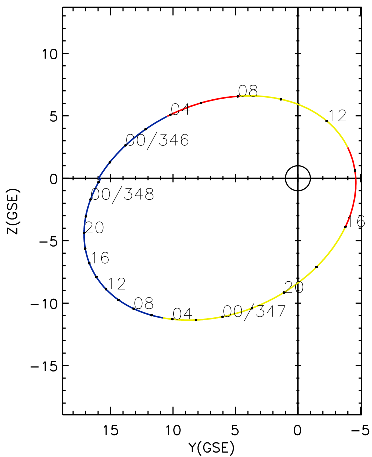
CLUSTER 2 orbit 2015 345 (12/11) 20:06 UT to 2015 348 (12/14) 02:26 UT
