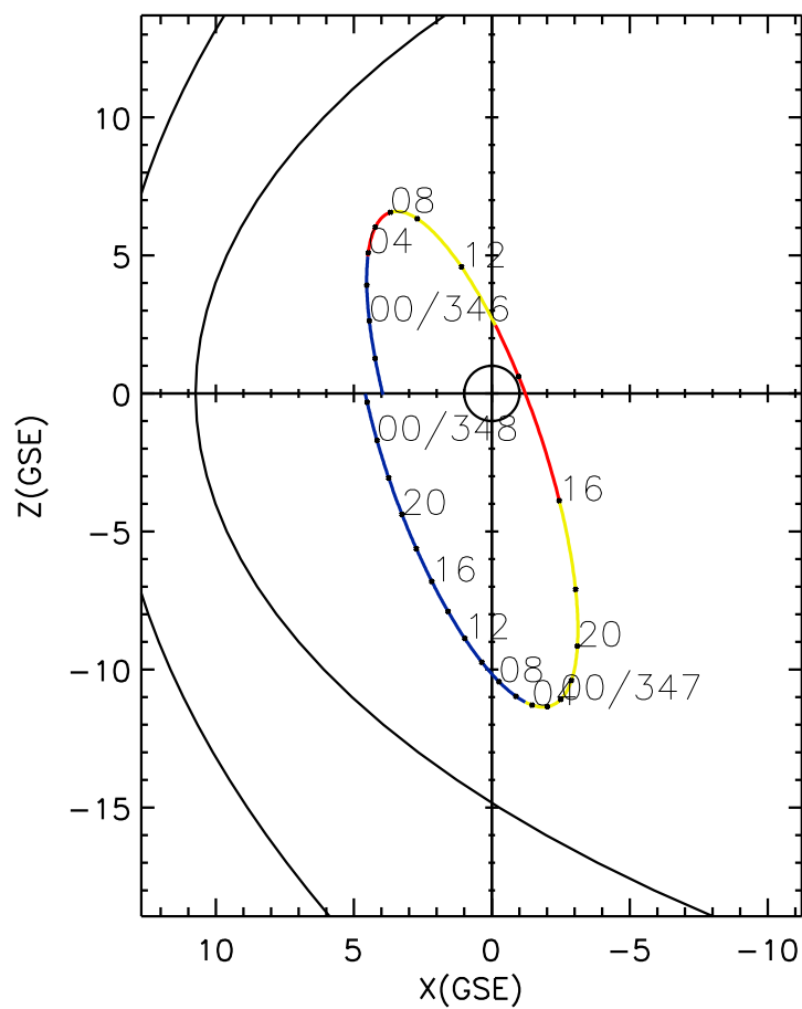
CLUSTER 2 orbit 2015 345 (12/11) 20:06 UT to 2015 348 (12/14) 02:26 UT
