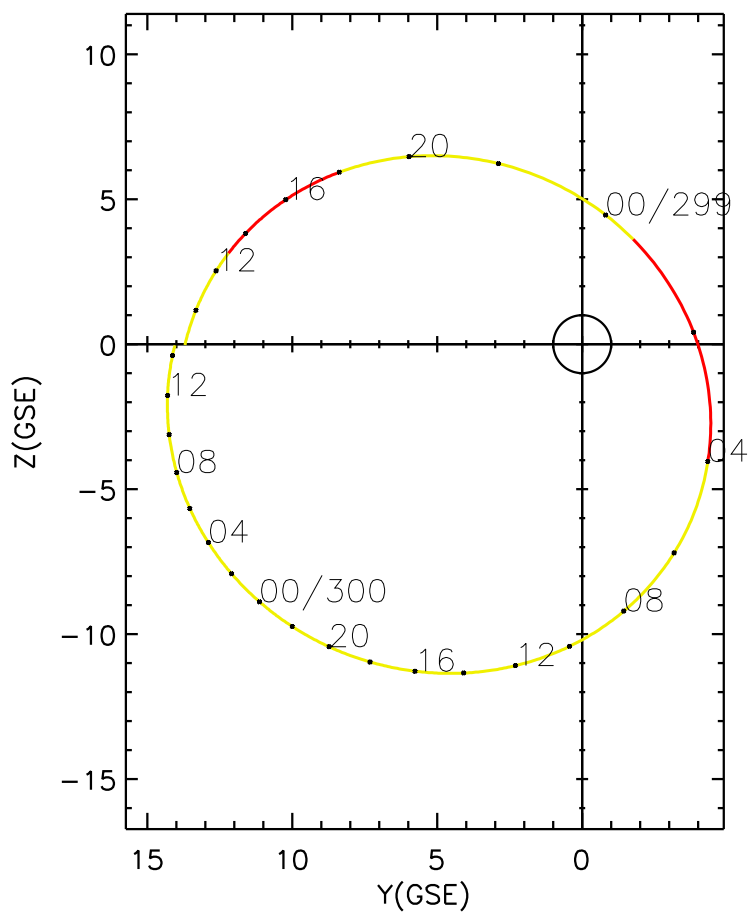
CLUSTER 2 orbit 2015 298 (10/25) 08:16 UT to 2015 300 (10/27) 14:31 UT
