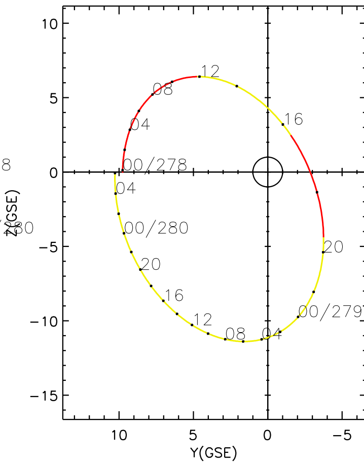
CLUSTER 2 orbit 2015 277 (10/04) 23:46 UT to 2015 280 (10/07) 06:06 UT
