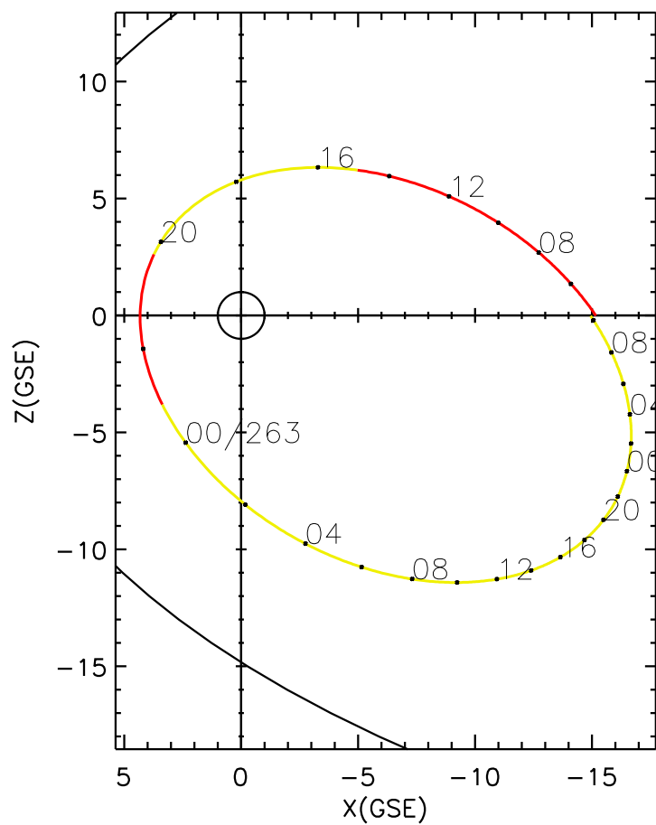
CLUSTER 2 orbit 2015 262 (09/19) 04:01 UT to 2015 264 (09/21) 10:16 UT
