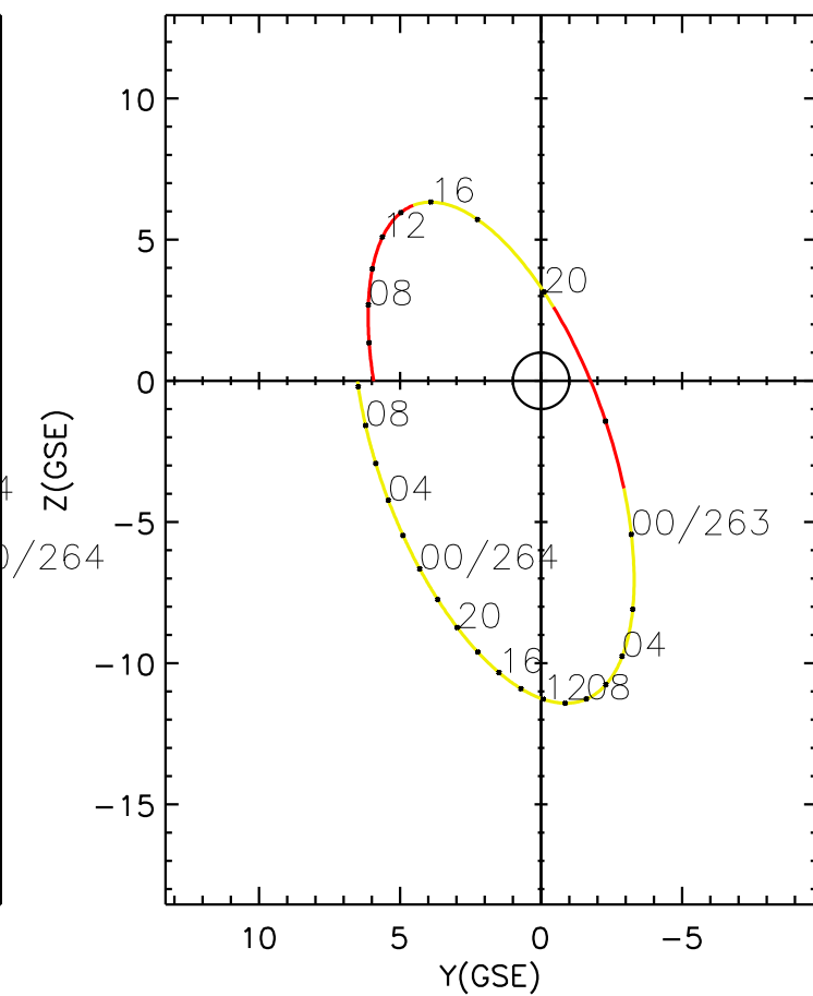
CLUSTER 2 orbit 2015 262 (09/19) 04:01 UT to 2015 264 (09/21) 10:16 UT
