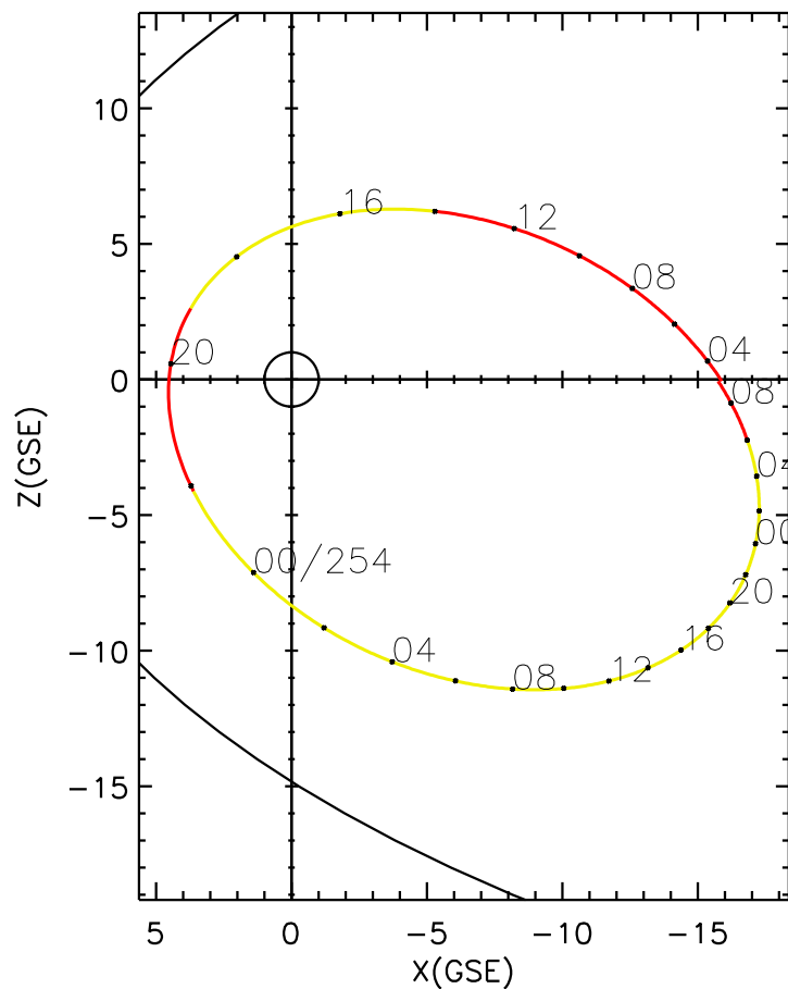
CLUSTER 2 orbit 2015 253 (09/10) 02:56 UT to 2015 255 (09/12) 09:11 UT
