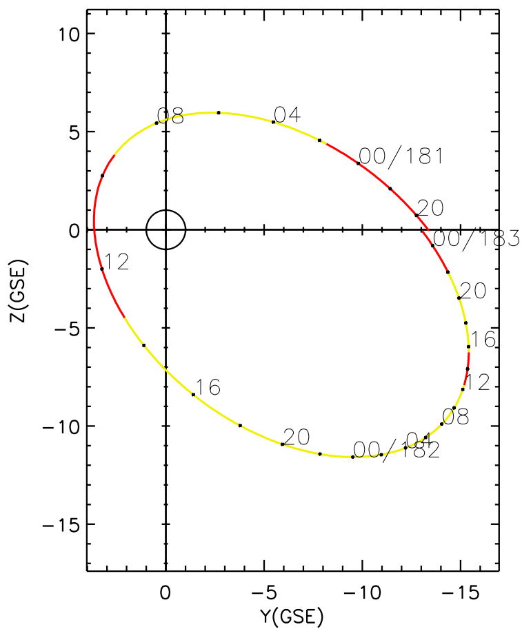
CLUSTER 2 orbit 2015 180 (06/29) 18:51 UT to 2015 183 (07/02) 01:06 UT
