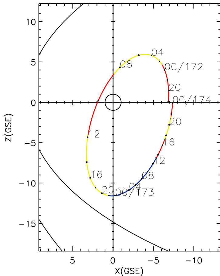
CLUSTER 2 orbit 2015 171 (06/20) 17:51 UT to 2015 174 (06/23) 00:06 UT
