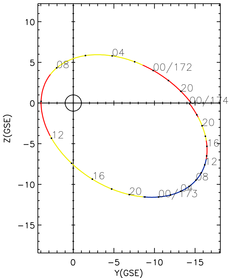
CLUSTER 2 orbit 2015 171 (06/20) 17:51 UT to 2015 174 (06/23) 00:06 UT
