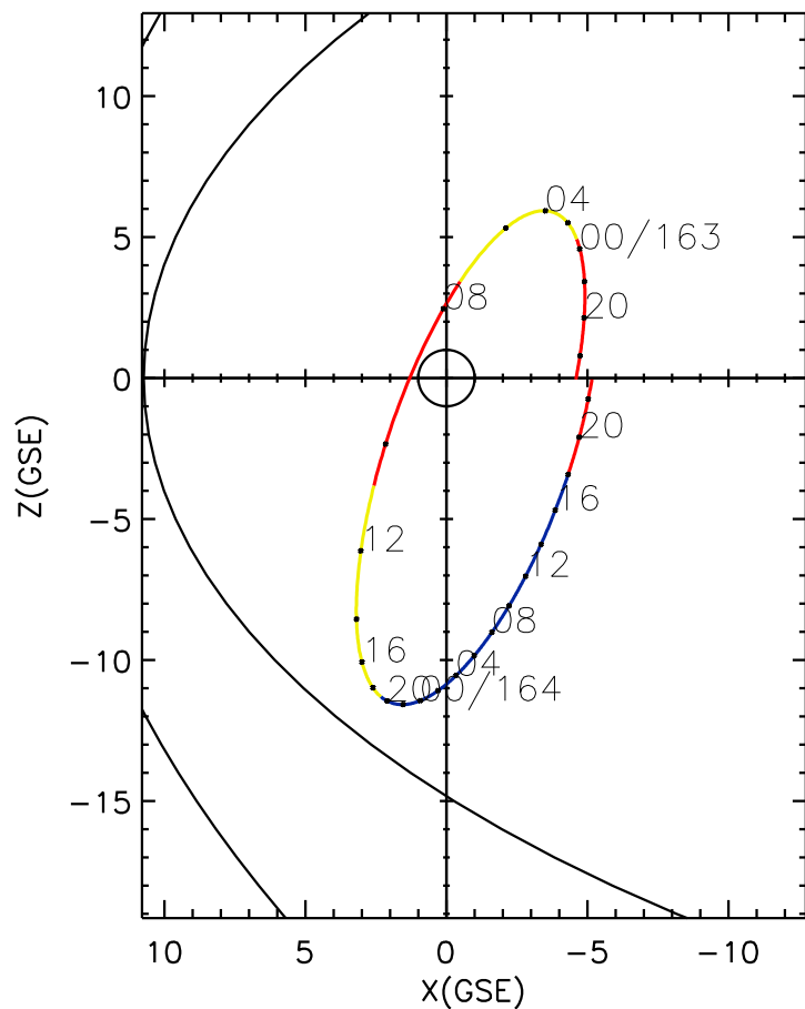
CLUSTER 2 orbit 2015 162 (06/11) 16:46 UT to 2015 164 (06/13) 23:01 UT
