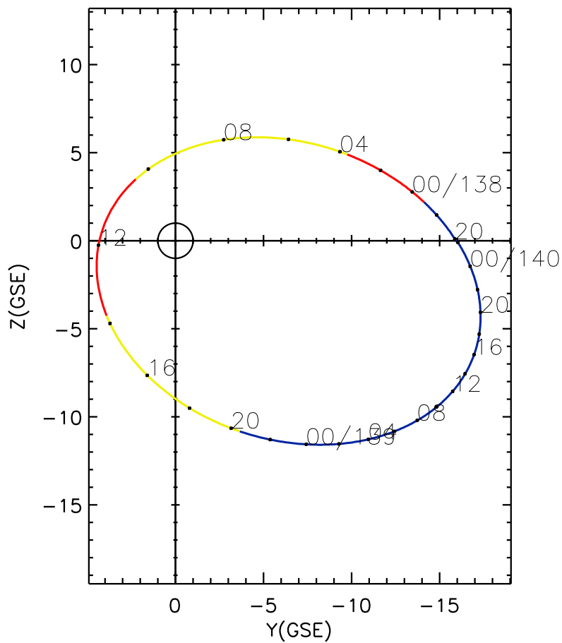
CLUSTER 2 orbit 2015 137 (05/17) 19:46 UT to 2015 140 (05/20) 02:06 UT
