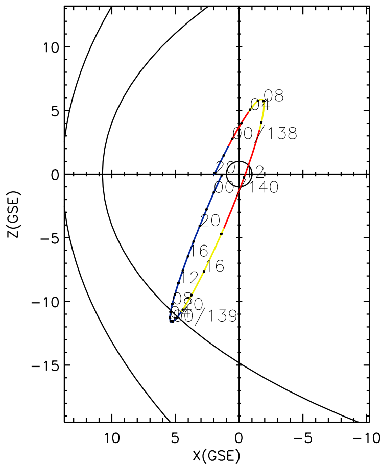
CLUSTER 2 orbit 2015 137 (05/17) 19:46 UT to 2015 140 (05/20) 02:06 UT
