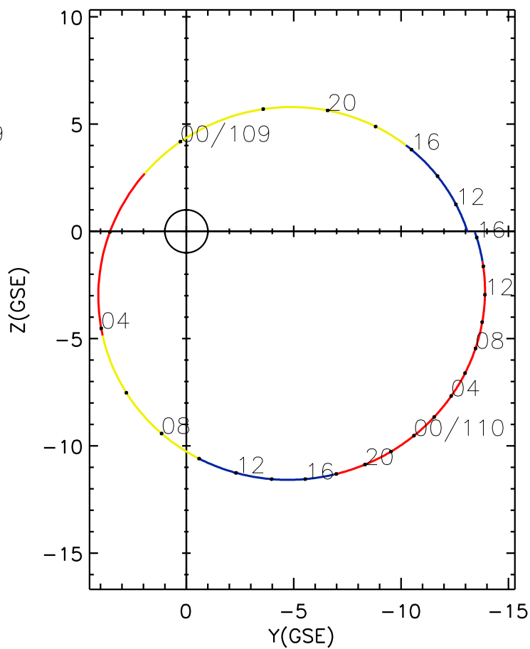
CLUSTER 2 orbit 2015 108 (04/18) 10:06 UT to 2015 110 (04/20) 16:21 UT
