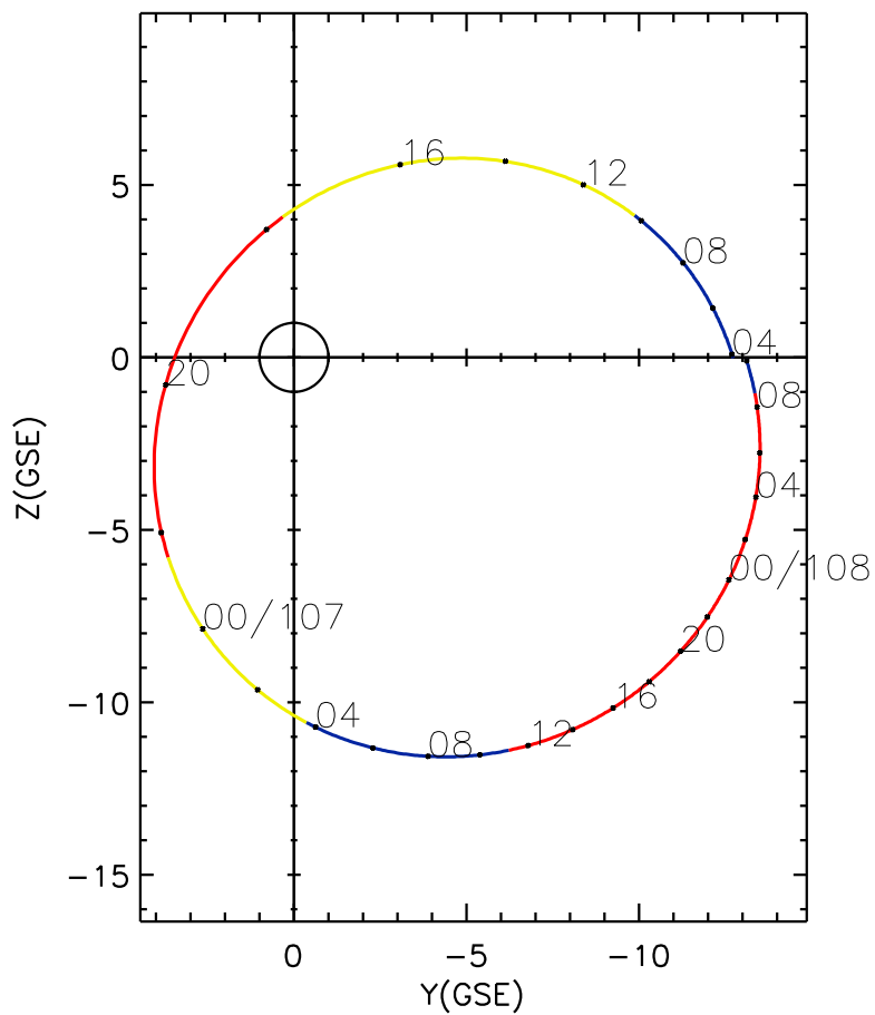
CLUSTER 2 orbit 2015 106 (04/16) 03:51 UT to 2015 108 (04/18) 10:06 UT
