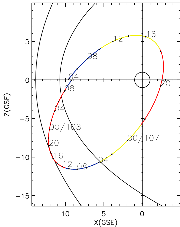
CLUSTER 2 orbit 2015 106 (04/16) 03:51 UT to 2015 108 (04/18) 10:06 UT
