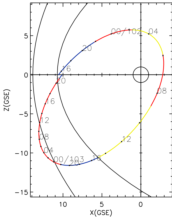
CLUSTER 2 orbit 2015 101 (04/11) 15:16 UT to 2015 103 (04/13) 21:36 UT
