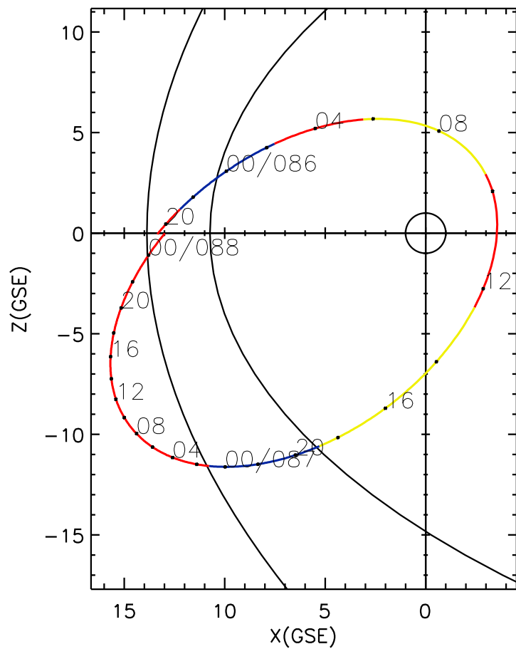
CLUSTER 2 orbit 2015 085 (03/26) 19:16 UT to 2015 088 (03/29) 01:36 UT
