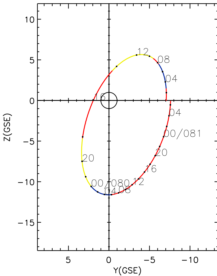
CLUSTER 2 orbit 2015 079 (03/20) 00:31 UT to 2015 081 (03/22) 06:46 UT
