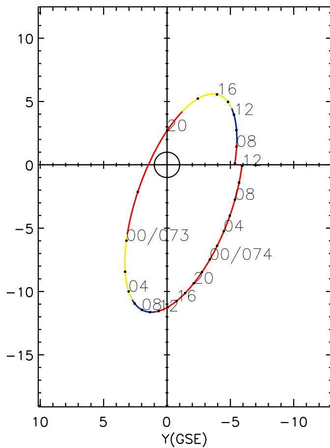
CLUSTER 2 orbit 2015 072 (03/13) 05:46 UT to 2015 074 (03/15) 12:01 UT
