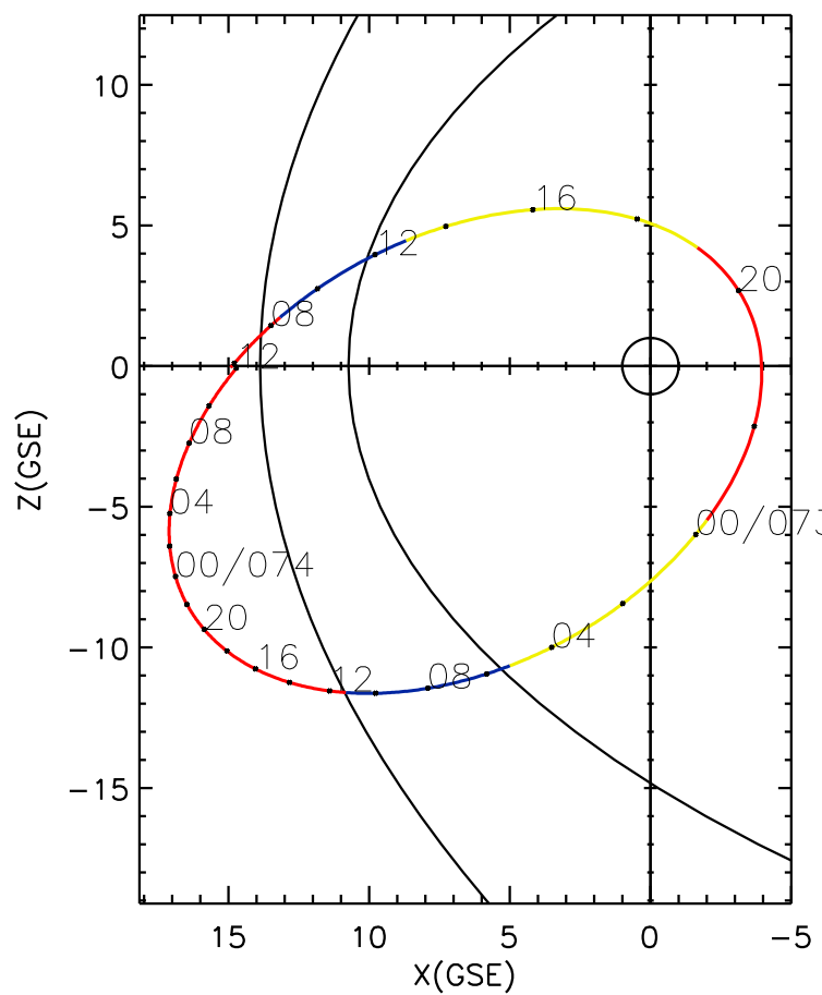
CLUSTER 2 orbit 2015 072 (03/13) 05:46 UT to 2015 074 (03/15) 12:01 UT
