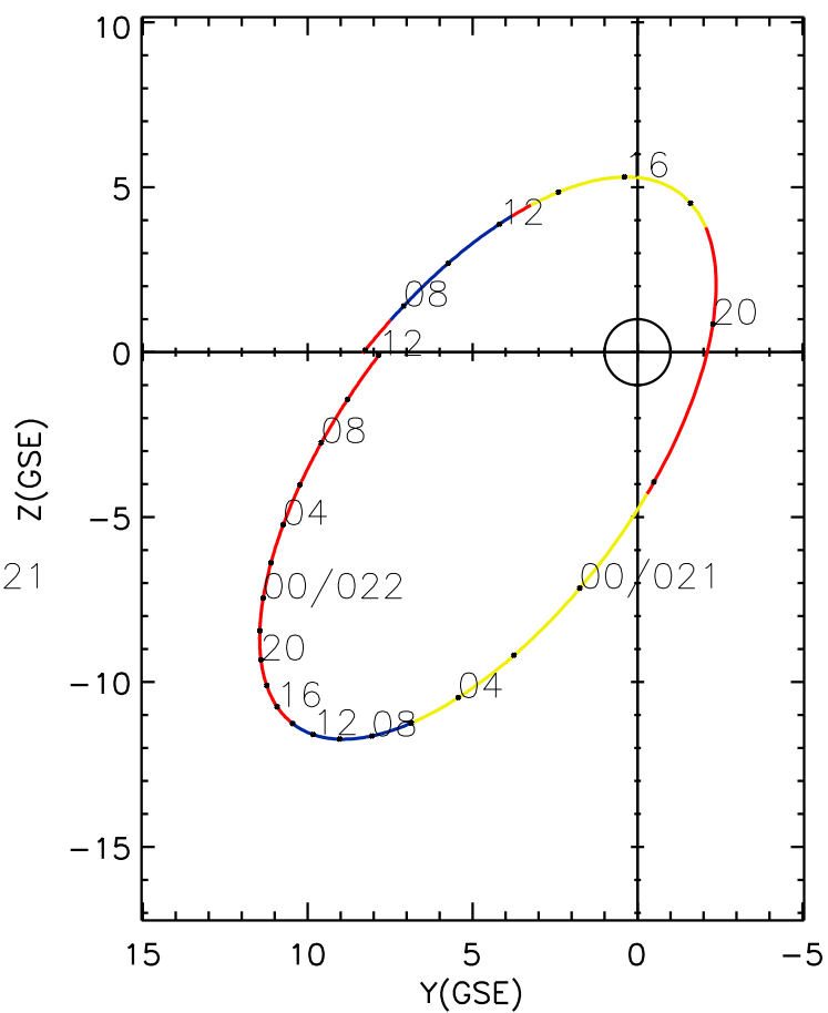
CLUSTER 2 orbit 2015 020 (01/20) 05:51 UT to 2015 022 (01/22) 12:06 UT
