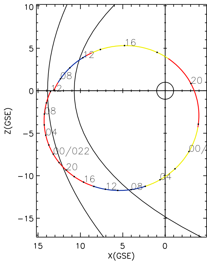
CLUSTER 2 orbit 2015 020 (01/20) 05:51 UT to 2015 022 (01/22) 12:06 UT
