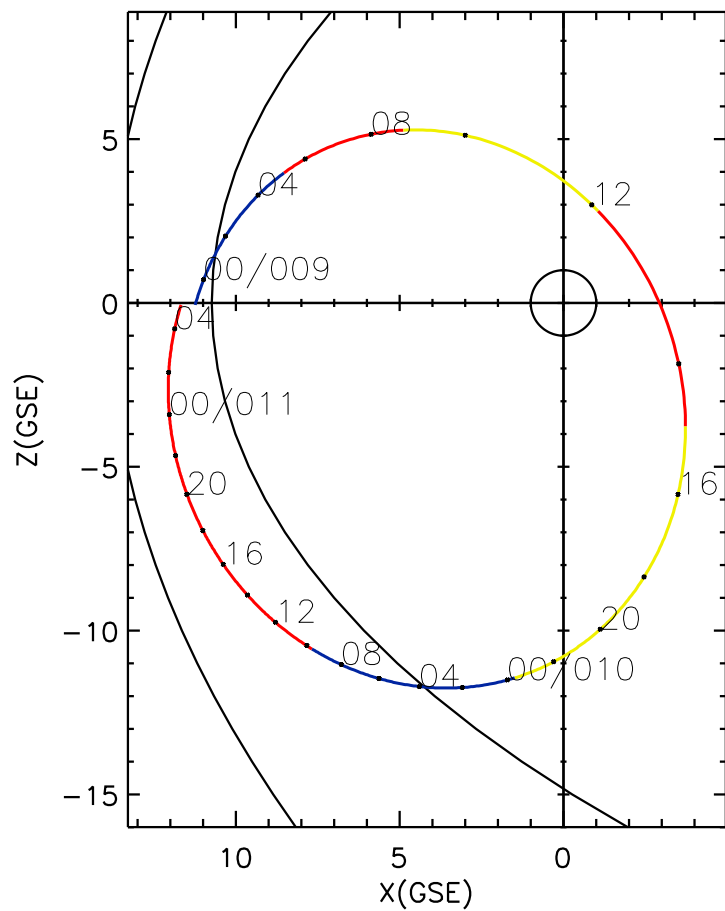
CLUSTER 2 orbit 2015 008 (01/08) 22:51 UT to 2015 011 (01/11) 05:06 UT
