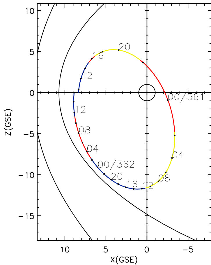
CLUSTER 2 orbit 2014 360 (12/26) 09:26 UT to 2014 362 (12/28) 15:36 UT
