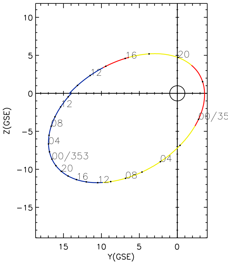
CLUSTER 2 orbit 2014 351 (12/17) 08:21 UT to 2014 353 (12/19) 14:41 UT
