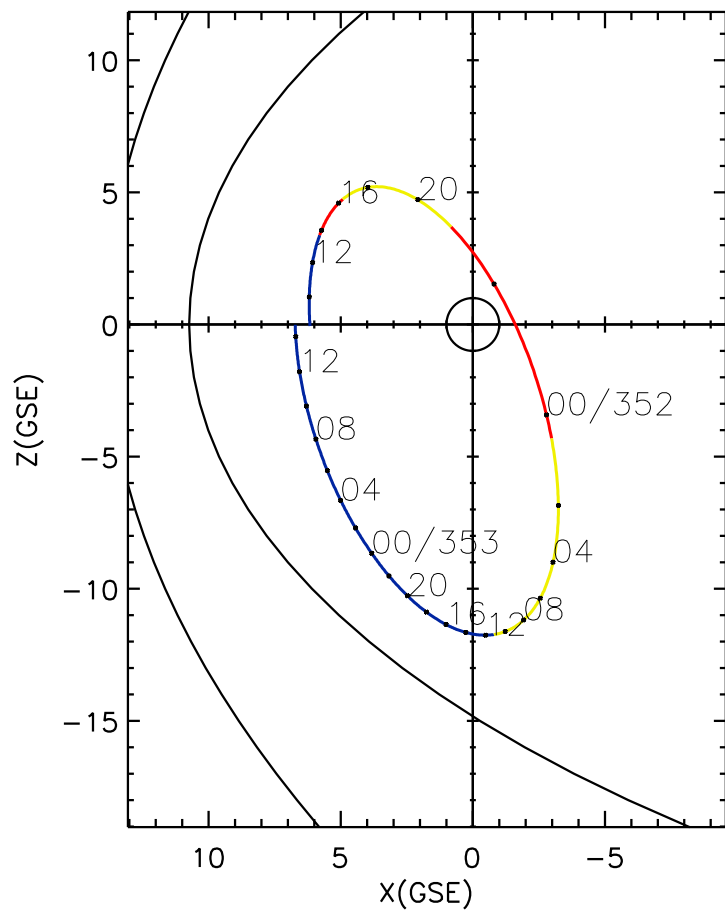
CLUSTER 2 orbit 2014 351 (12/17) 08:21 UT to 2014 353 (12/19) 14:41 UT
