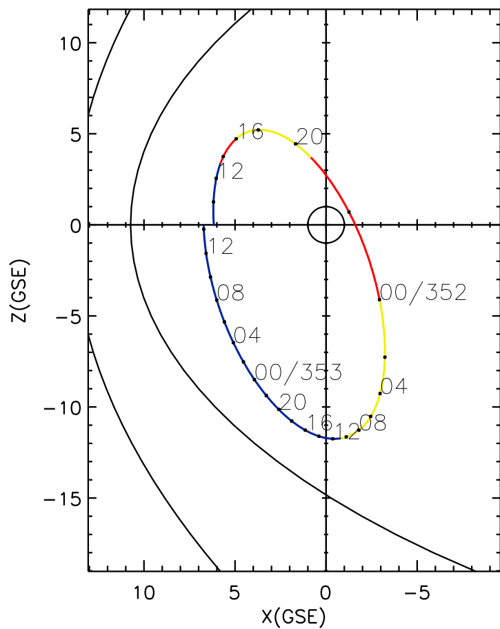
CLUSTER 2 orbit 2014 351 (12/17) 08:01 UT to 2014 353 (12/19) 14:21 UT
