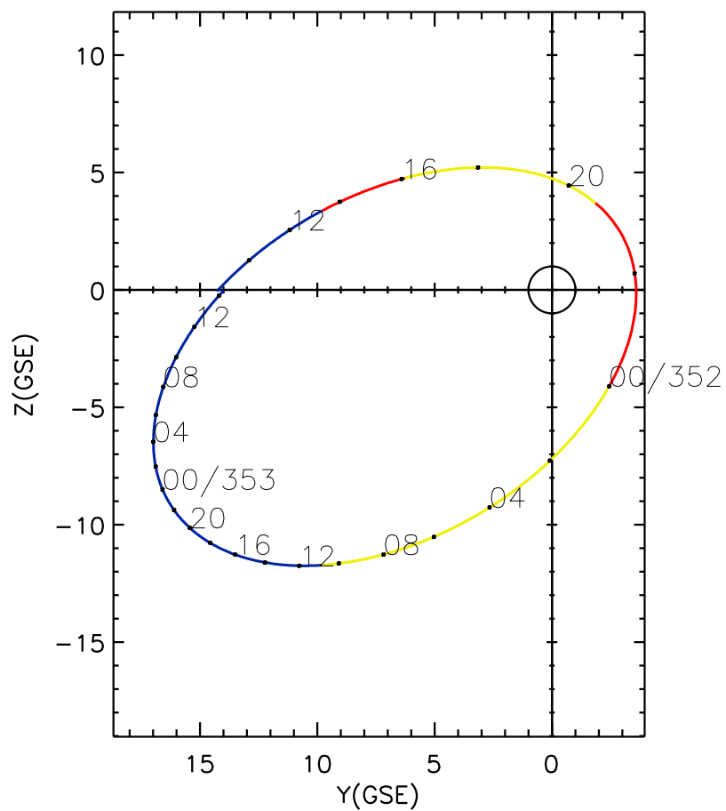
CLUSTER 2 orbit 2014 351 (12/17) 08:01 UT to 2014 353 (12/19) 14:21 UT
