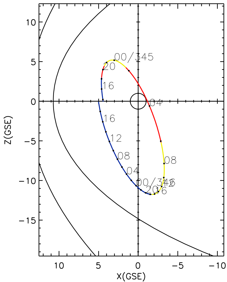
CLUSTER 2 orbit 2014 344 (12/10) 13:36 UT to 2014 346 (12/12) 19:51 UT
