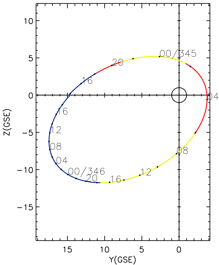
CLUSTER 2 orbit 2014 344 (12/10) 13:36 UT to 2014 346 (12/12) 19:51 UT
