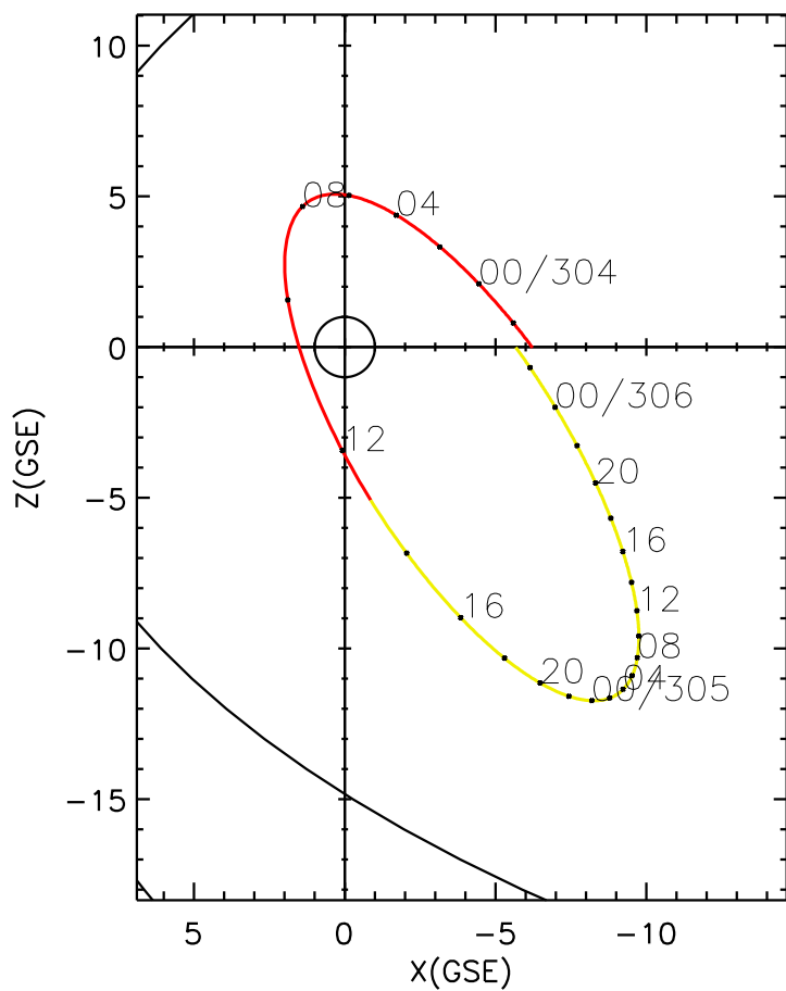
CLUSTER 2 orbit 2014 303 (10/30) 20:46 UT to 2014 306 (11/02) 03:01 UT
