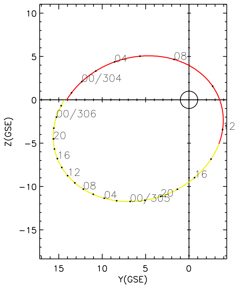
CLUSTER 2 orbit 2014 303 (10/30) 20:46 UT to 2014 306 (11/02) 03:01 UT
