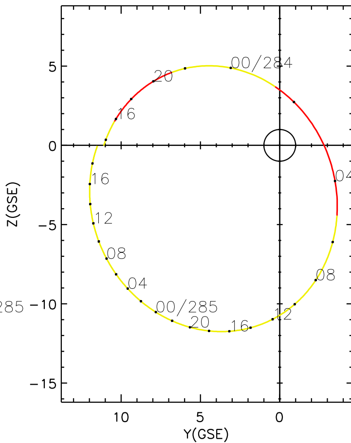
CLUSTER 2 orbit 2014 283 (10/10) 13:26 UT to 2014 285 (10/12) 19:41 UT
