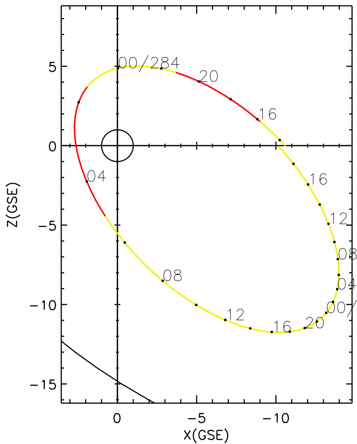
CLUSTER 2 orbit 2014 283 (10/10) 13:26 UT to 2014 285 (10/12) 19:41 UT
