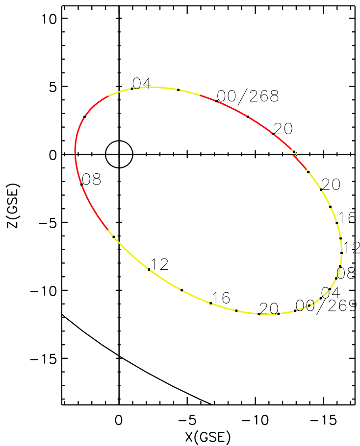
CLUSTER 2 orbit 2014 267 (09/24) 17:41 UT to 2014 269 (09/26) 23:56 UT
