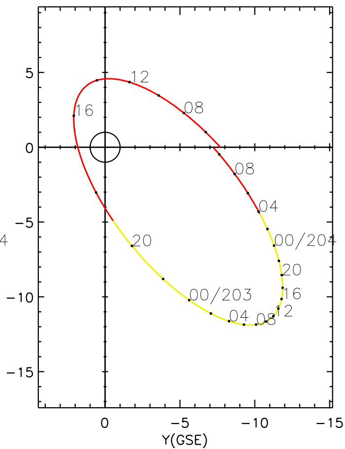
CLUSTER 2 orbit 2014 202 (07/21) 04:26 UT to 2014 204 (07/23) 10:41 UT
