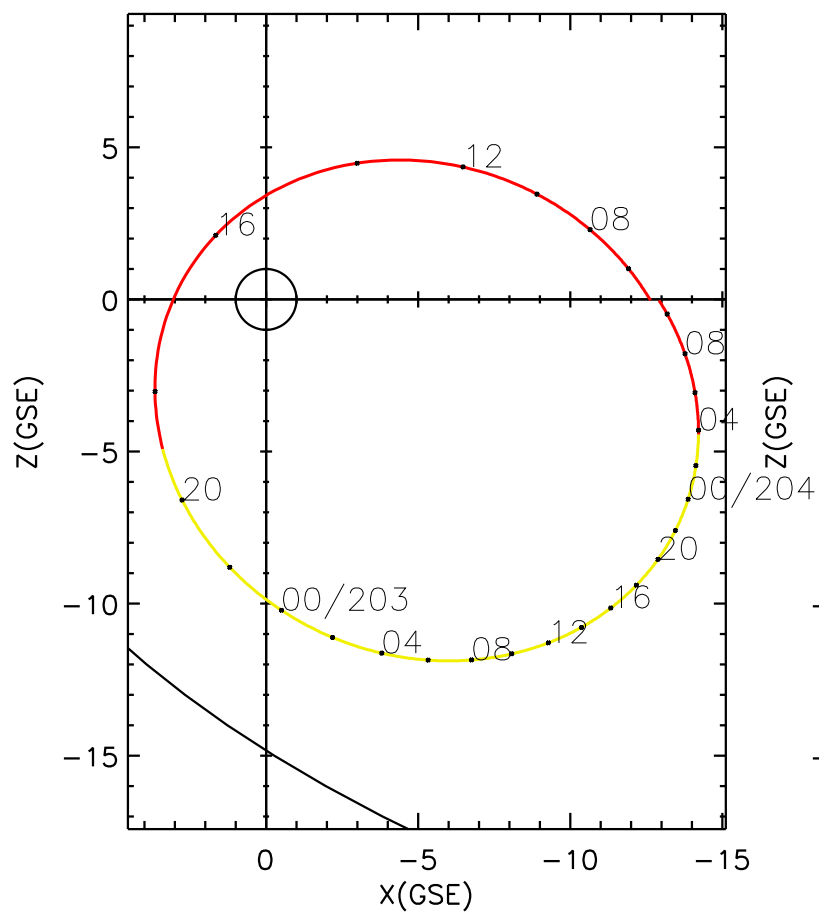
CLUSTER 2 orbit 2014 202 (07/21) 04:26 UT to 2014 204 (07/23) 10:41 UT
