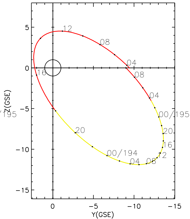
CLUSTER 2 orbit 2014 193 (07/12) 03:26 UT to 2014 195 (07/14) 09:41 UT
