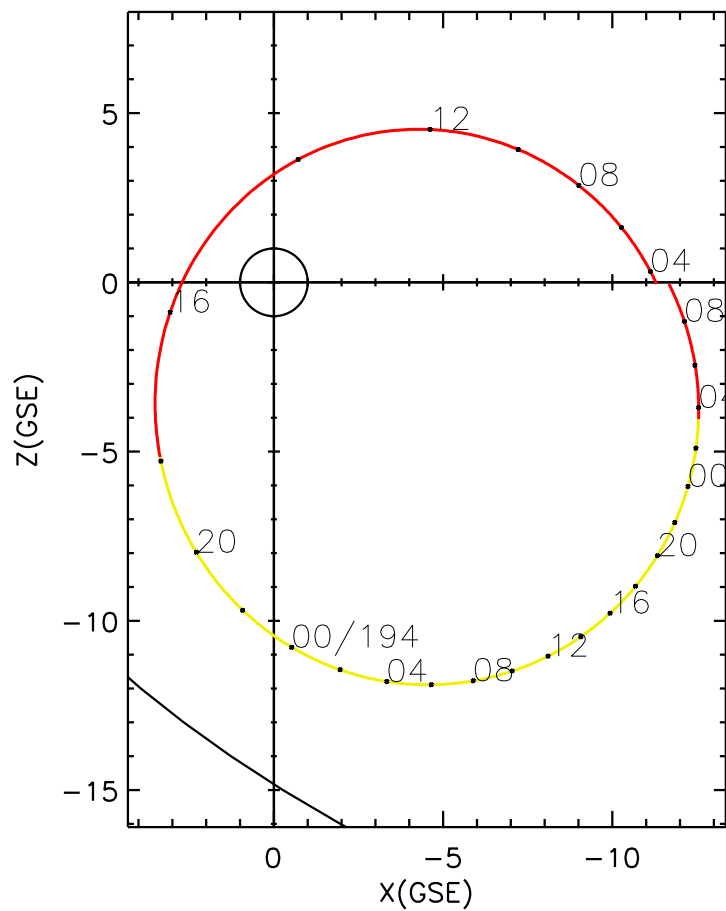
CLUSTER 2 orbit 2014 193 (07/12) 03:26 UT to 2014 195 (07/14) 09:41 UT
