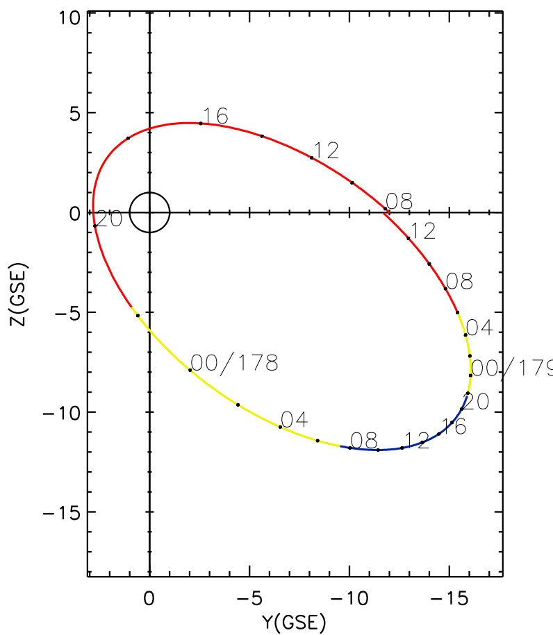
CLUSTER 2 orbit 2014 177 (06/26) 07:41 UT to 2014 179 (06/28) 13:56 UT
