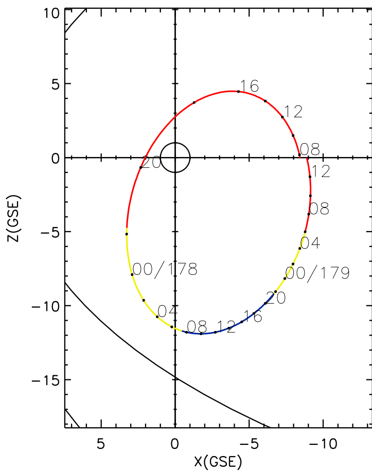
CLUSTER 2 orbit 2014 177 (06/26) 07:41 UT to 2014 179 (06/28) 13:56 UT
