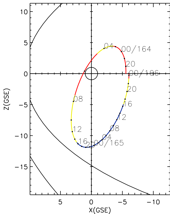
CLUSTER 2 orbit 2014 163 (06/12) 18:11 UT to 2014 166 (06/15) 00:26 UT
