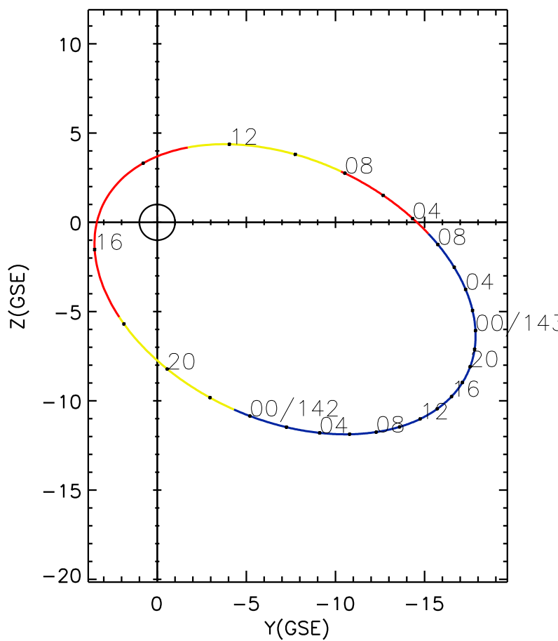
CLUSTER 2 orbit 2014 141 (05/21) 03:36 UT to 2014 143 (05/23) 09:51 UT
