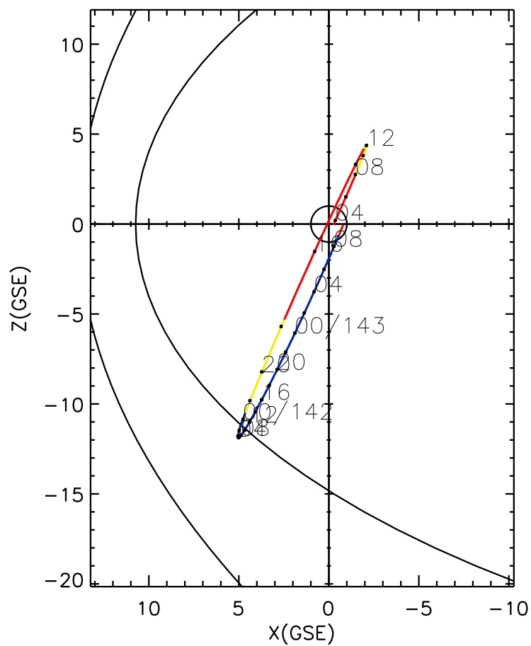
CLUSTER 2 orbit 2014 141 (05/21) 03:36 UT to 2014 143 (05/23) 09:51 UT
