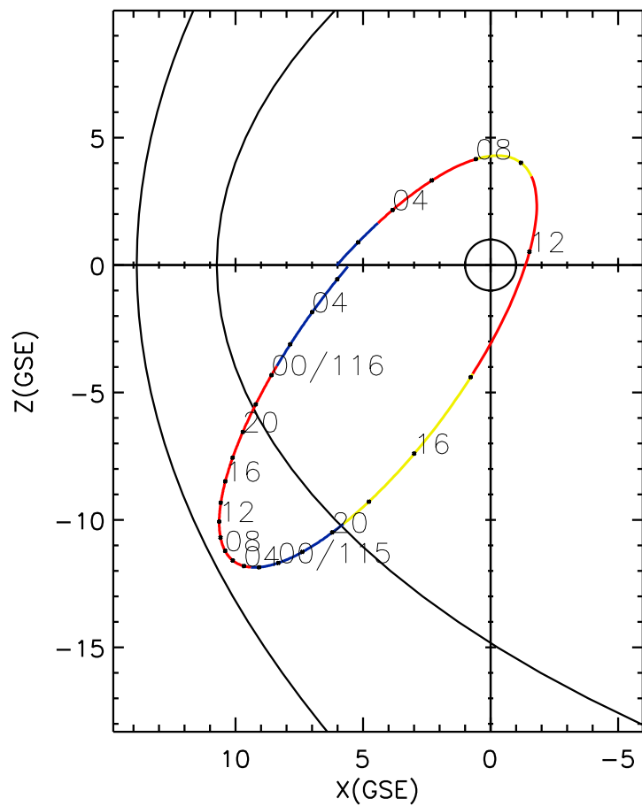
CLUSTER 2 orbit 2014 114 (04/24) 00:36 UT to 2014 116 (04/26) 06:46 UT
