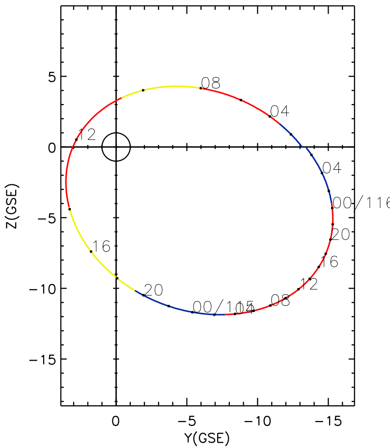
CLUSTER 2 orbit 2014 114 (04/24) 00:36 UT to 2014 116 (04/26) 06:46 UT
