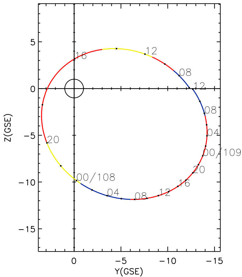
CLUSTER 2 orbit 2014 107 (04/17) 05:51 UT to 2014 109 (04/19) 12:06 UT
