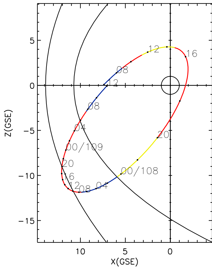
CLUSTER 2 orbit 2014 107 (04/17) 05:51 UT to 2014 109 (04/19) 12:06 UT
