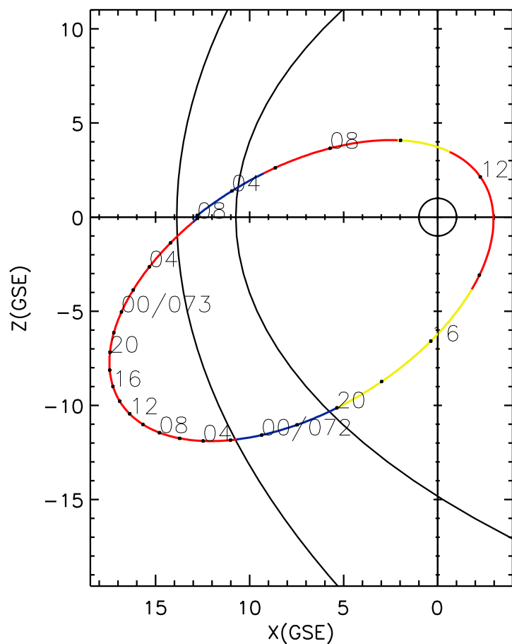
CLUSTER 2 orbit 2014 071 (03/12) 01:51 UT to 2014 073 (03/14) 08:06 UT
